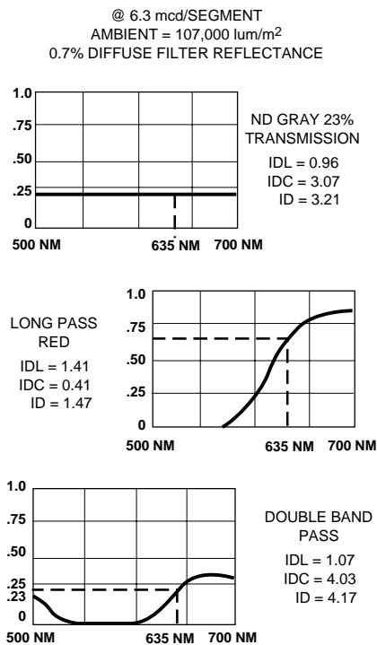
Figure 29. HDSP-3530 High Efficiency Red 0.30 inch Display.
