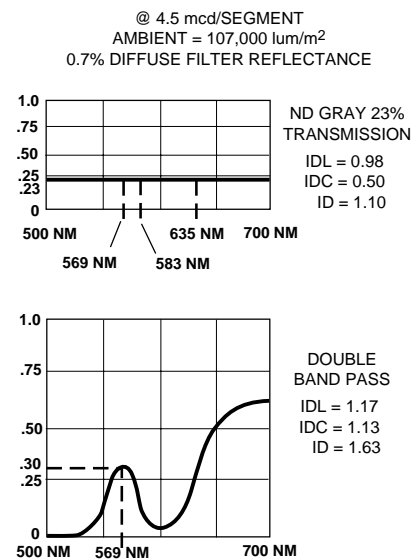
Figure 31. HDSP Green 0.30 inch Display.
