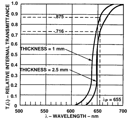
Figure 4. Variation in Relative Transmittance vs. Thickness for a Constant Density Filter Material.
