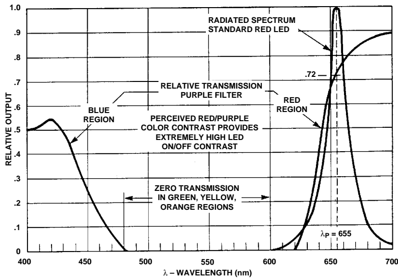
Figure 13. A Purple Color Wavelength Filter for Standard Red LED Displays.
