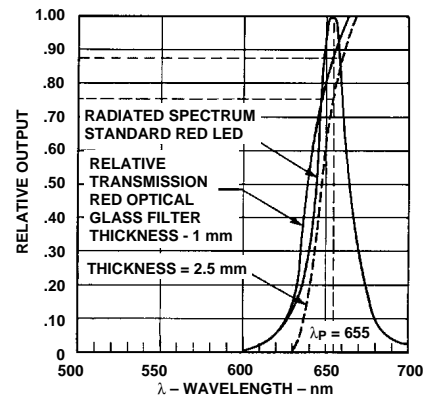
Figure 15. A Red Optical Glass Filter for use with High Efficiency Red LED Displays.
