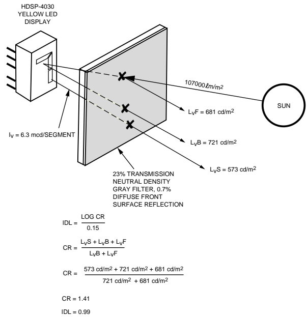
Figure 25. Luminance Index — Diffuse Front Surface Reflectance.
