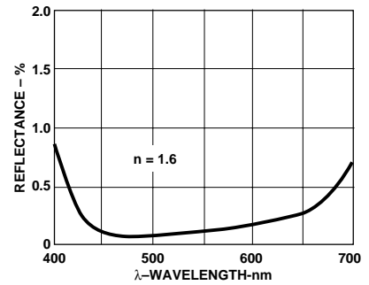
Figure 36. Front Surface Reflectance of Glass with Double Sided 1/4 Wave Optical Coating.
