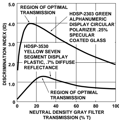
Figure 46. Optimal Neutral Density Gray Filter Transmission.
