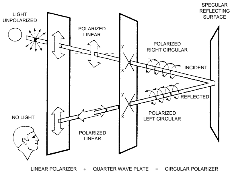
Figure 35. Operation of a Circular Polarizer.
