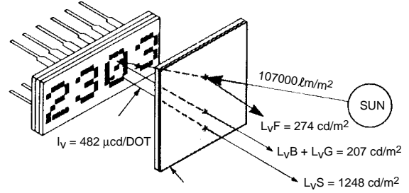
HDSP-2303 GREEN DISPLAY
