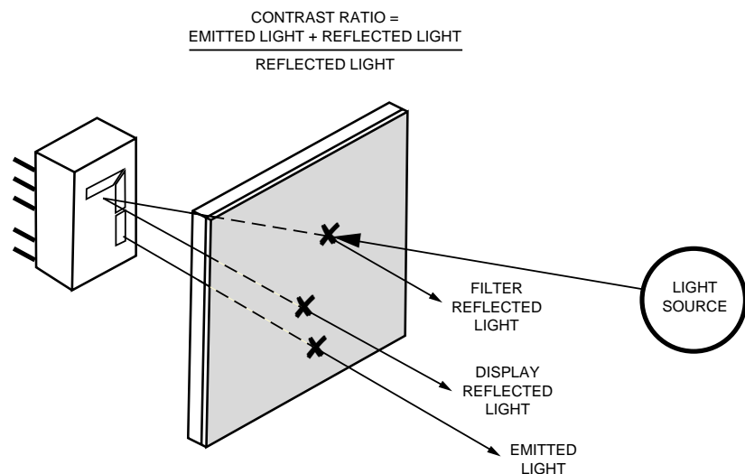
Figure 5. Luminance Contrast for a Light Emitting Display with a Filter.
