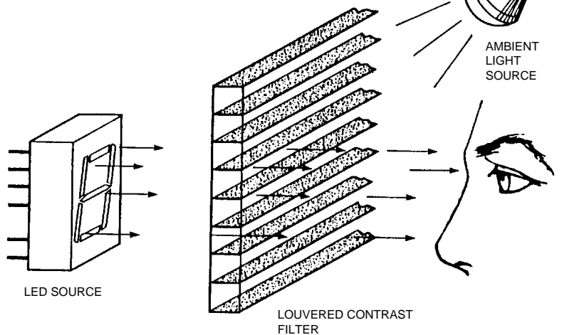
Figure 32. The Operation of a Louvered Filter.
