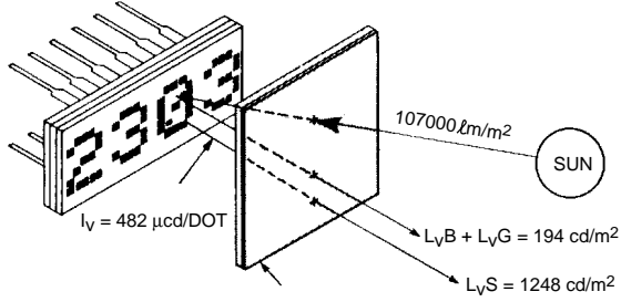
HDSP-2303 GREEN DISPLAY
