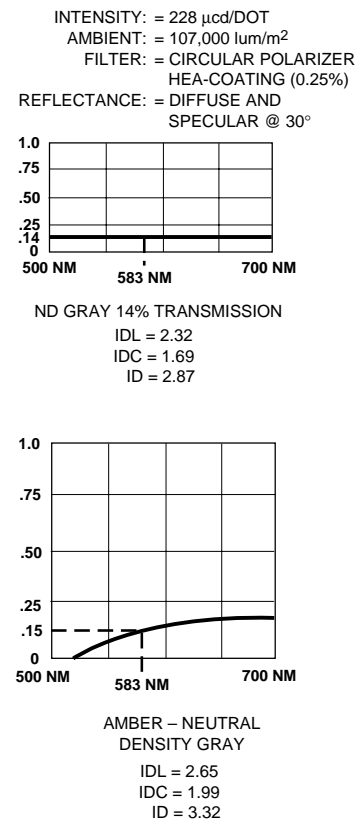
Figure 43. HDSP-2301 Yellow Alphanumeric 0.20 inch Display.
