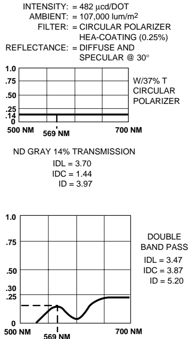
Figure 42. HDSP-2303 Green Alphanumeric 0.20 inch Display.
