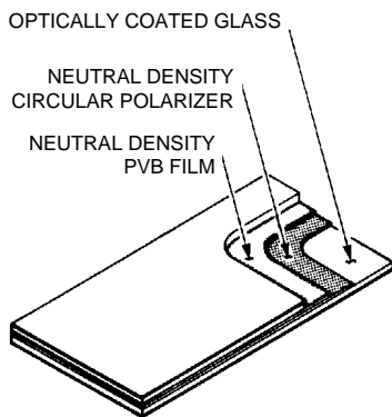
Figure 37. Circular Polarizer Laminated Between a Piece of HEA Coated Glass and a Piece of Uncoated Glass.
