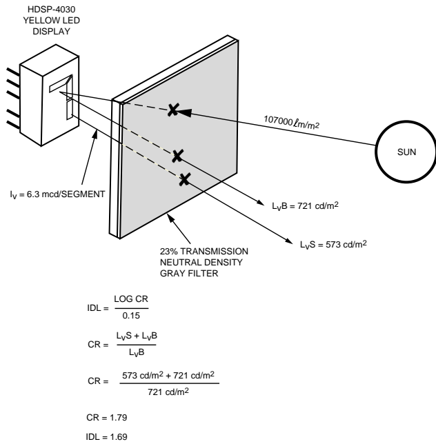
Figure 24. Luminance Index — No Front Surface Reflectance.
