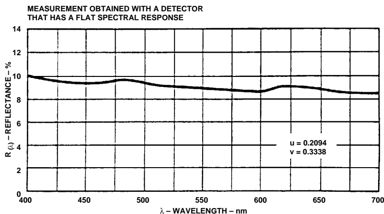
Figure 23. Reflectance Characteristic for the Face of a Gray Body Stretched Segment Sunlight Viewable LED Display.
