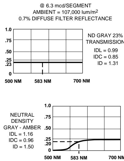
Figure 30. HDSP-4030 Yellow 0.30 inch Display.
