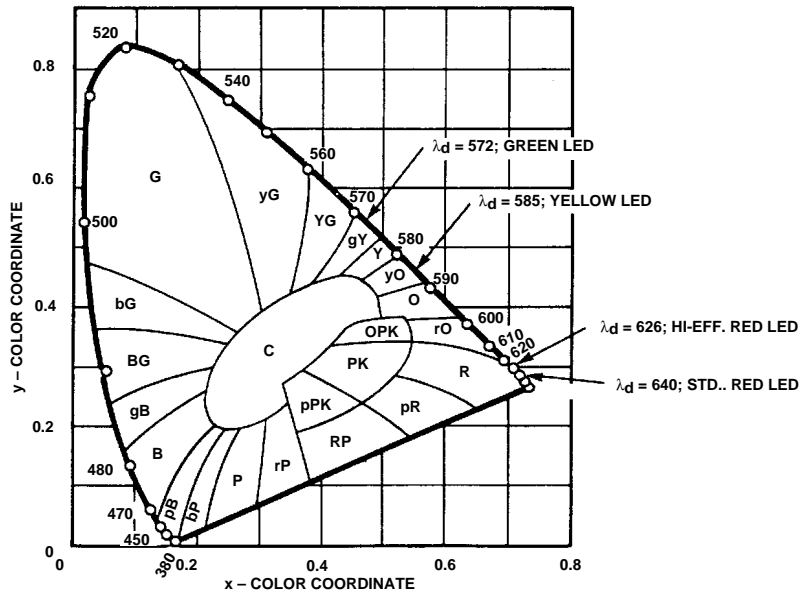
Figure 19. Dominant Wavelengths and Corresponding Colors for LEDs, Shown on the CIE Chromaticity Diagram.
