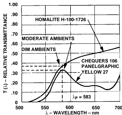
Figure 8. Typical Transmittance Curves for Filters to be used with Yellow Displays.
