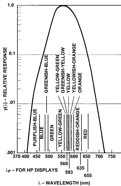
Figure 1. CIE Standard Observer Eye Response Curve (Photopic Curve), including CIE Vivid Color Ranges.
