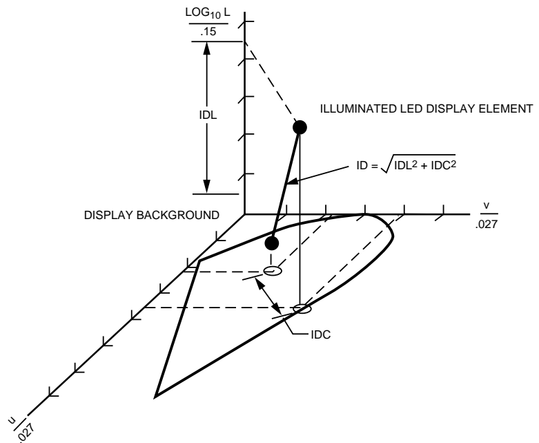
Figure 22. Photocolorimetric Space.
