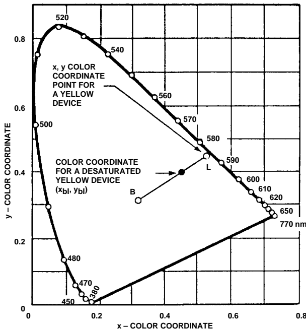
Figure 20. Additive Color Mixture.
