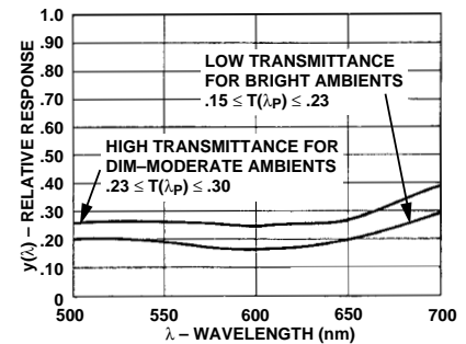
Figure 10. Typical Transmittance Curves for Filters to be used with All Colored Displays.
