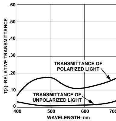
Figure 38. Spectral Characteristics of a Circular Polarizing Optically Coated Glass Filter.
