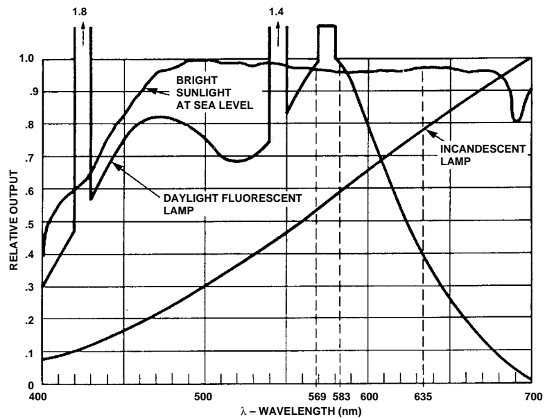
Figure 16. Spectral Distribution for Sunlight, Daylight Fluorescent and Incandescent Ambient Lighting.
