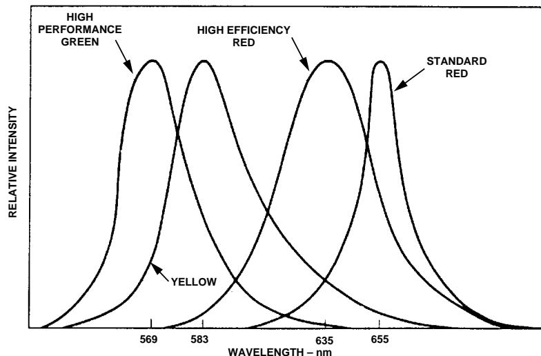
Figure 2. Relative Intensity vs. Wavelength.
