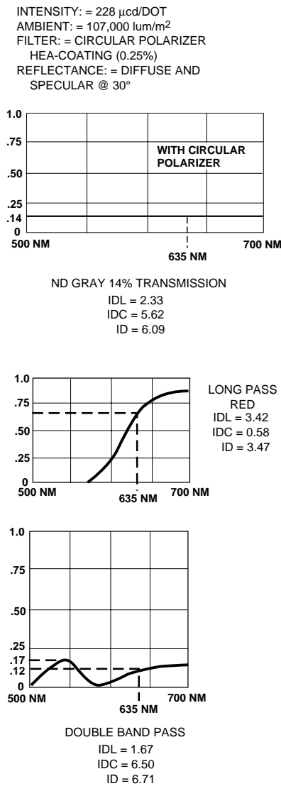
Figure 44. HDSP-2302 High Efficiency Red 0.20 inch Display.
