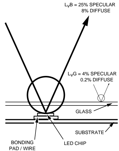
Figure 34. Dot Matrix Alphanumeric Display, Typical Values of Reflectance at 30°.
